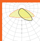
Lysfordeling ASYM 45°x140°
