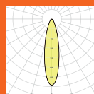
Lysfordeling SYM R30
