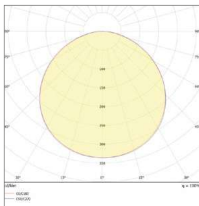
DOWNLIGHT SLIM
