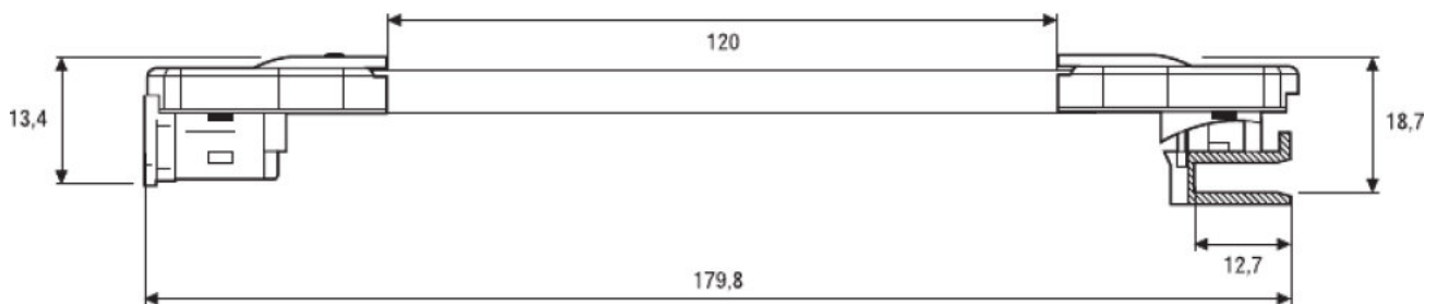
LF-4CONN PROT
