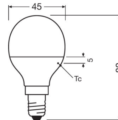
BASE CLAS P 40 FR 5.5 W/2700K E14, BASE CLAS P 40 FR 5.5 W/2700K E14, BASE CLAS P 40 FR 5.5 W/4000K E14
