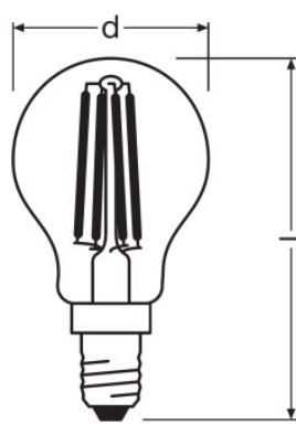
BASE CLAS P 40 4 W/2700K E14, BASE CLAS P 40 4 W/2700K E14, BASE CLAS P 40 4 W/4000K E14
