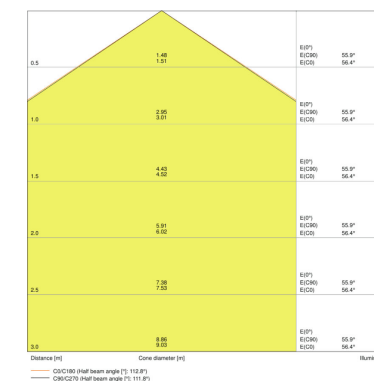
SF BLKH 300 S 15W/3000K BK IP65
