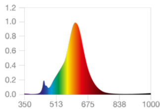
EPREL Data Spectral Diagram LEDr AC42289 2200K TW
