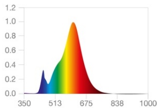
EPREL Data Spectral Diagram LEDr AC42294 2700K TW
