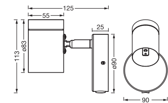
LED SPOT STAMP 1XGU10 WT
