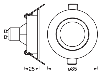
SP SET ADJCLICK3.7W827DIMGU10
