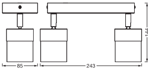
LED SPOT HALF WOOD LINE 2XGU10 WT
