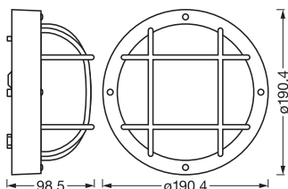
BULKHEAD ESSENTIAL ROUND
